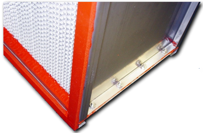
Close-up of TRI-PURE™ HEPA HT frame media pack and sealant
